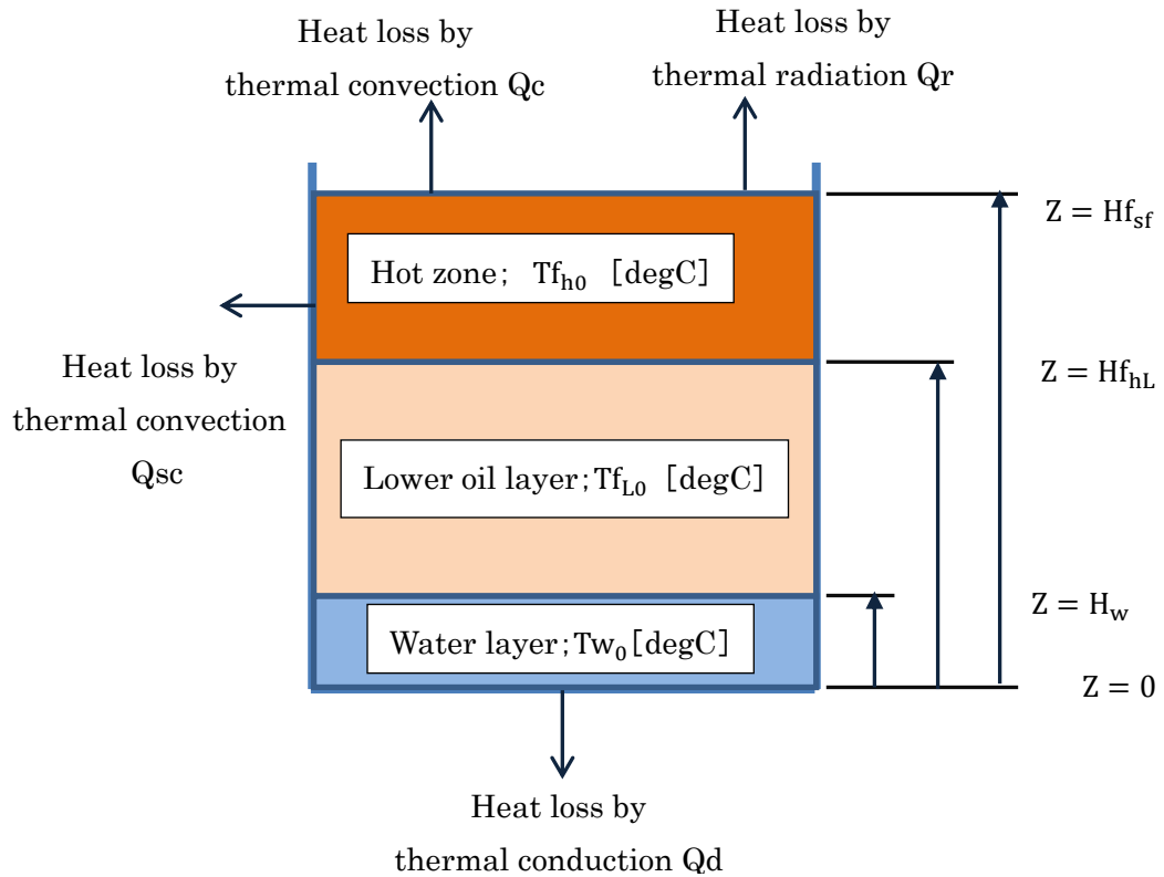
Fig 5 Calculation model of the temperature profile after extinguishment of a crude oil tank fire.
