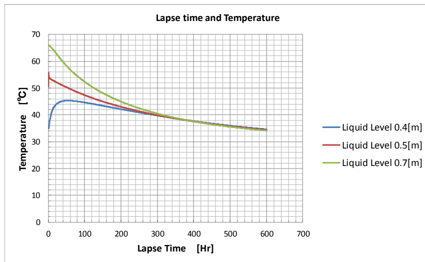
Fig. -8 Temperature profile of oil after extinguishment in case of cooling the tank wall by water stream, case 4
