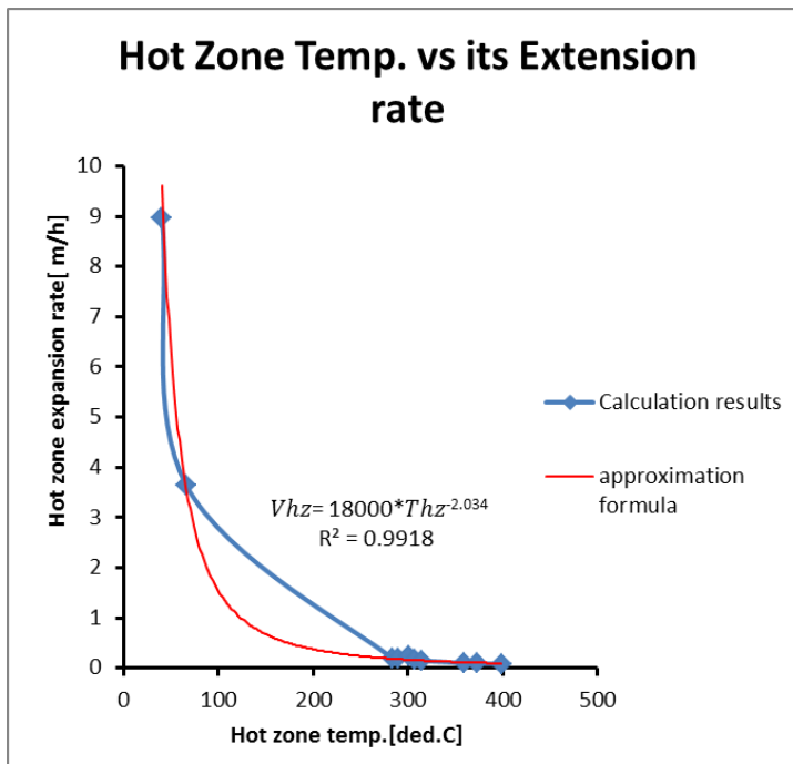
Fig. -3 Relation between hot zone temperature and hot zone extension rate
