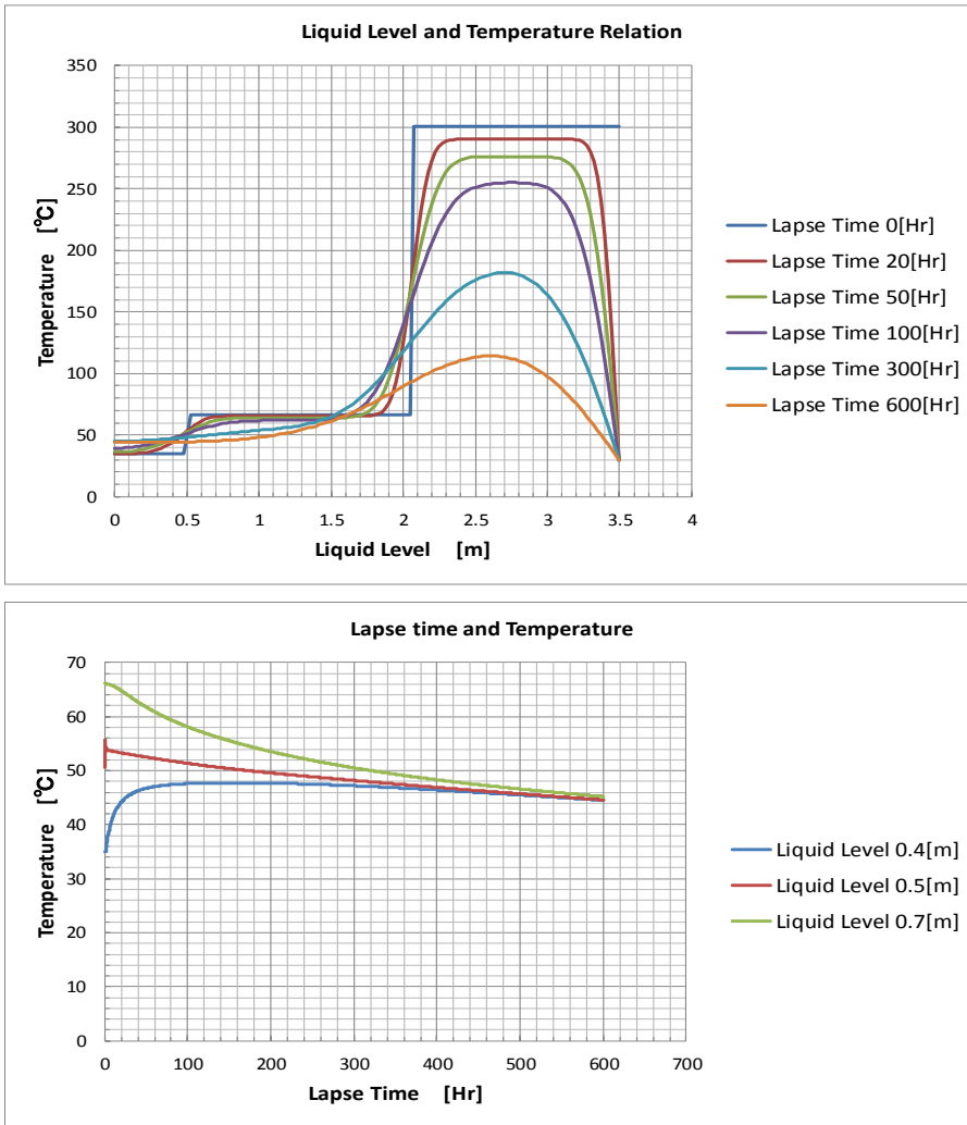
Fig. -7 Temperature profile of oil after extinguishment in case of cooling the tank wall by wind, case 4
