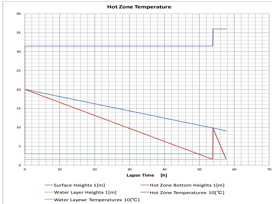
Fig. 4 Crude Oil No.– 3, Temperature at the boilover is assumed to be 350 [degC]. The distillation cycle proceeds and the hot zone temperature is increased to 359.6 [degC]. from 314.4 [degC].
