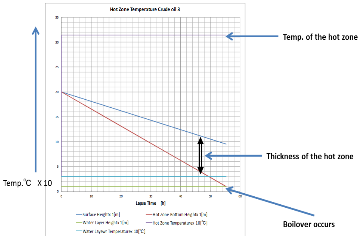
Fig. 2 The hot zone calculation results for the crude oil No. -2 and 3
