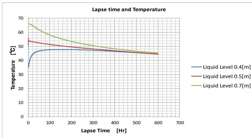
Fig. -7 Temperature profile of oil after extinguishment in case of cooling the tank wall by wind, case 4
