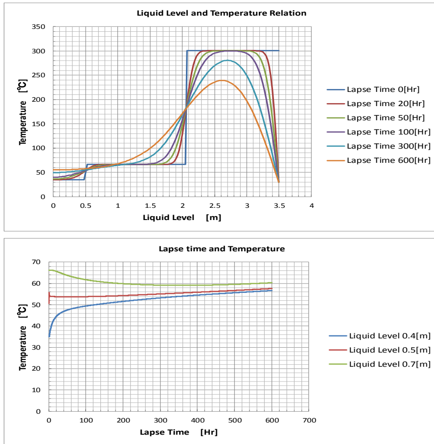
Fig. -6 Temperature profile of oil after extinguishment in case of no heat loss from the tank wall, case 4
