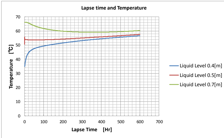
Fig. -6 Temperature profile of oil after extinguishment in case of no heat loss from the tank wall, case4
