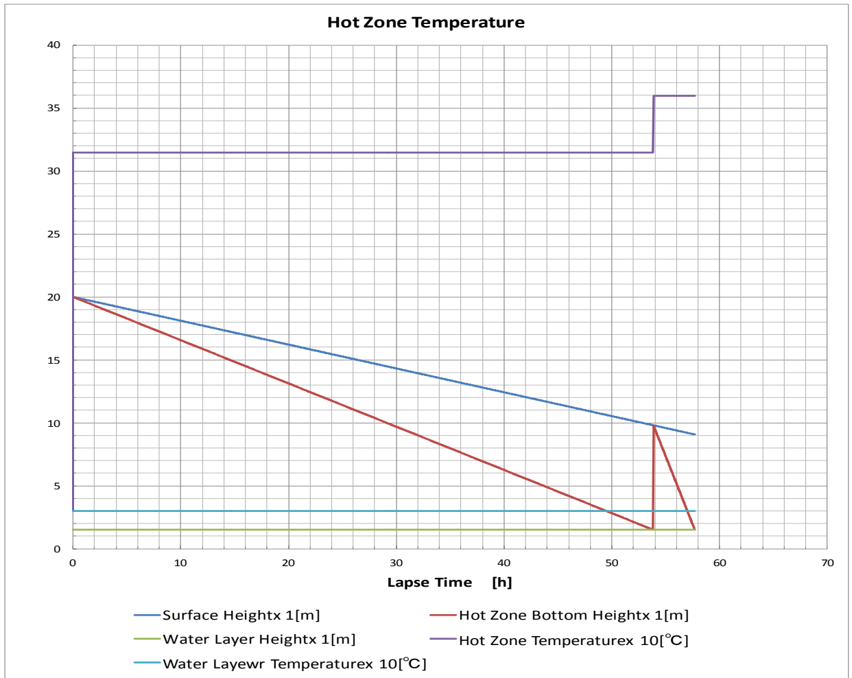
Fig. 4 Crude Oil No.- 3, Temperature at the boilover is assumed to be 350 [degC]. The distillation cycle proceeds and the hot zone temperature is increased to 359.6 [degC], from 314.4 [degC].
