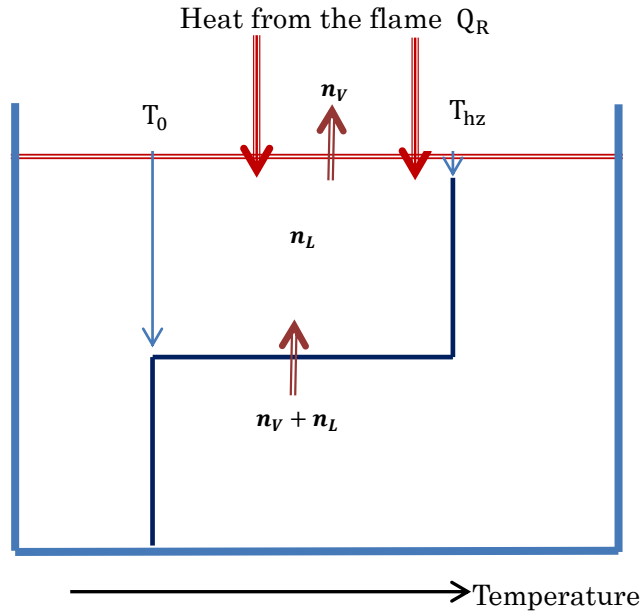
Fig. 1 Theoretical model of the hot zone formation in case of a crude oil tank fire
