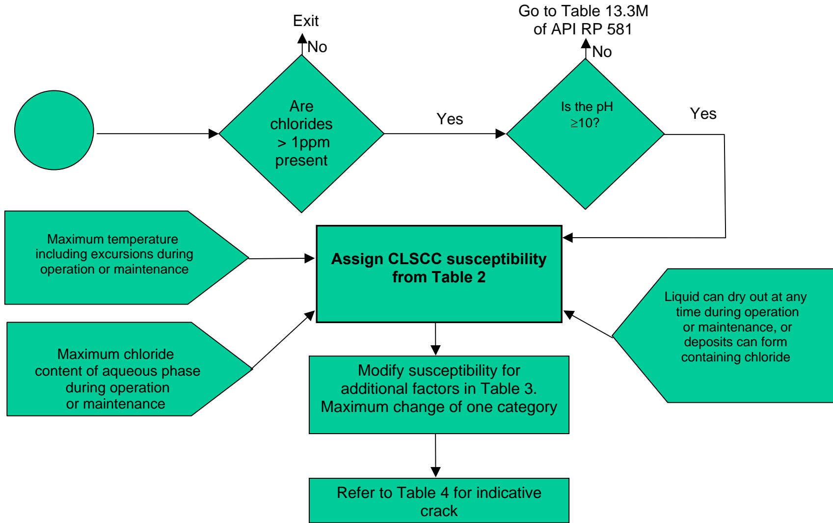
Figure 2. Proposed extension of susceptibility assessment for CLSCC in API RP 581, Part 2, section 13.
