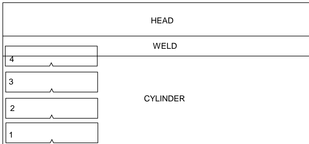
Figure 3. The positions of the fracture toughness specimens
