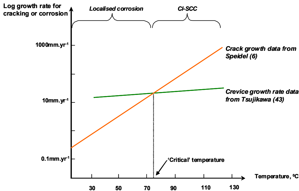
Figure 1. Schematic graph to demonstrate the competition concept proposed by Tsujikawa [43]. Note how changes in crack growth rate or corrosion rate can alter the ‘critical’ temperature for CLSCC.
