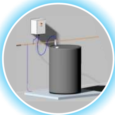
Example of correct grounding technique for a static dissipative drum
