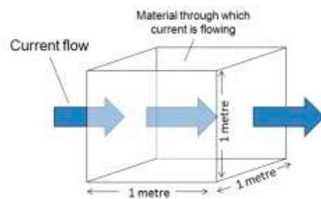
Resistance experienced by current flowing through material is influenced by the resistivity value, \rho , for the material and the length and cross-sectional area of the material.
