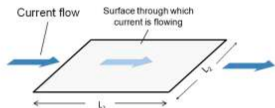
Resistance experienced by current flowing across surface is influenced by the surface resistivity value, \lambda , of the material and the length and breadth of the material.
